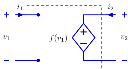
VCVS i_1 = 0 v_2 = f(v_1)
