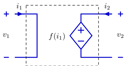
CCVS v_1 = 0 v_2 = f(i_1)
